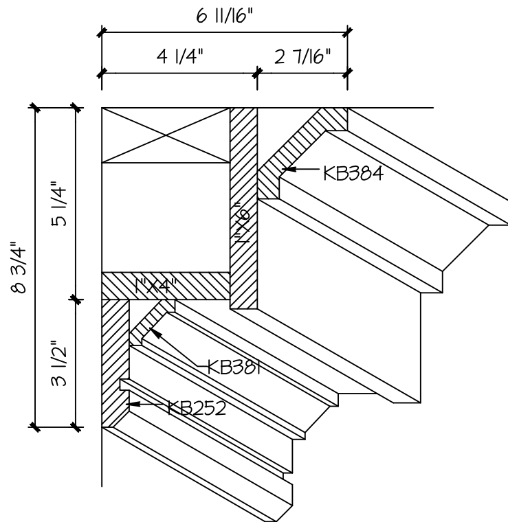
WALL BEAM
